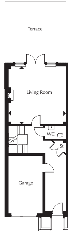
Ground Floor
